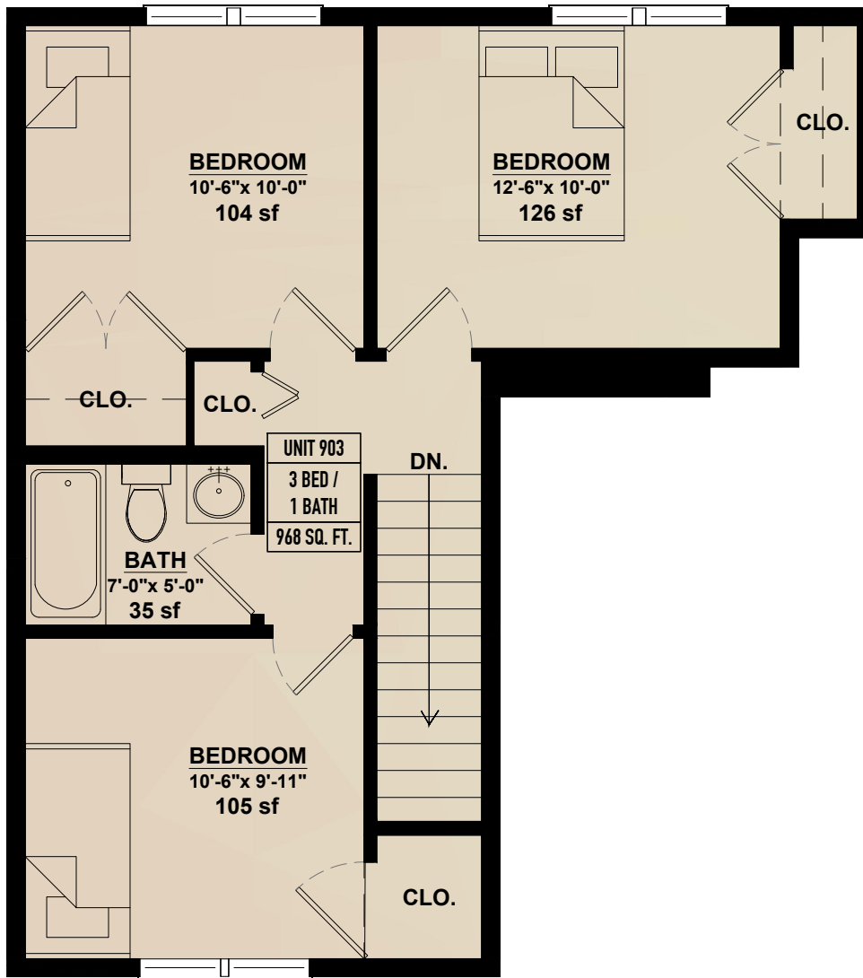
SECOND FLOOR
