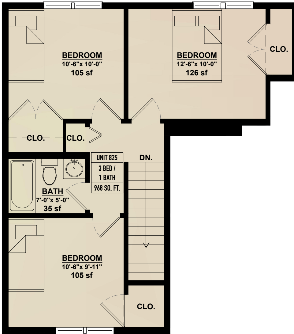
SECOND FLOOR
