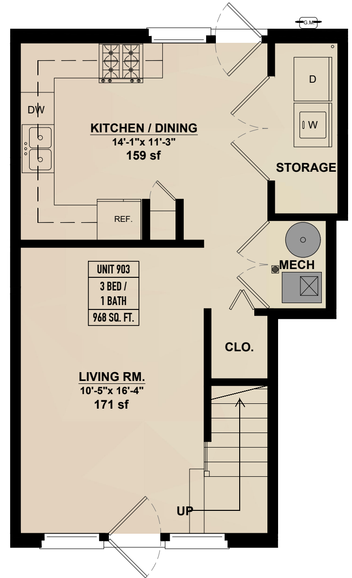
GROUND FLOOR
