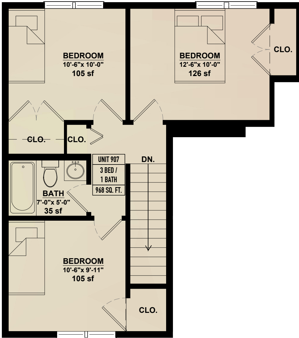
SECOND FLOOR
