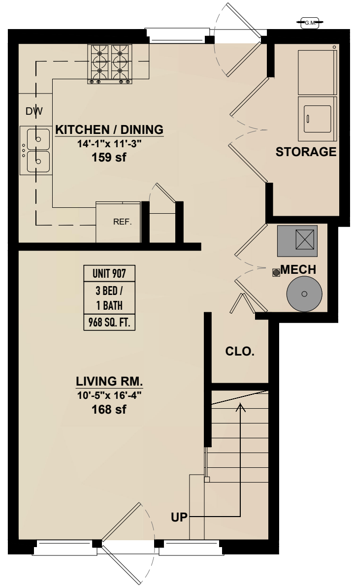
GROUND FLOOR
