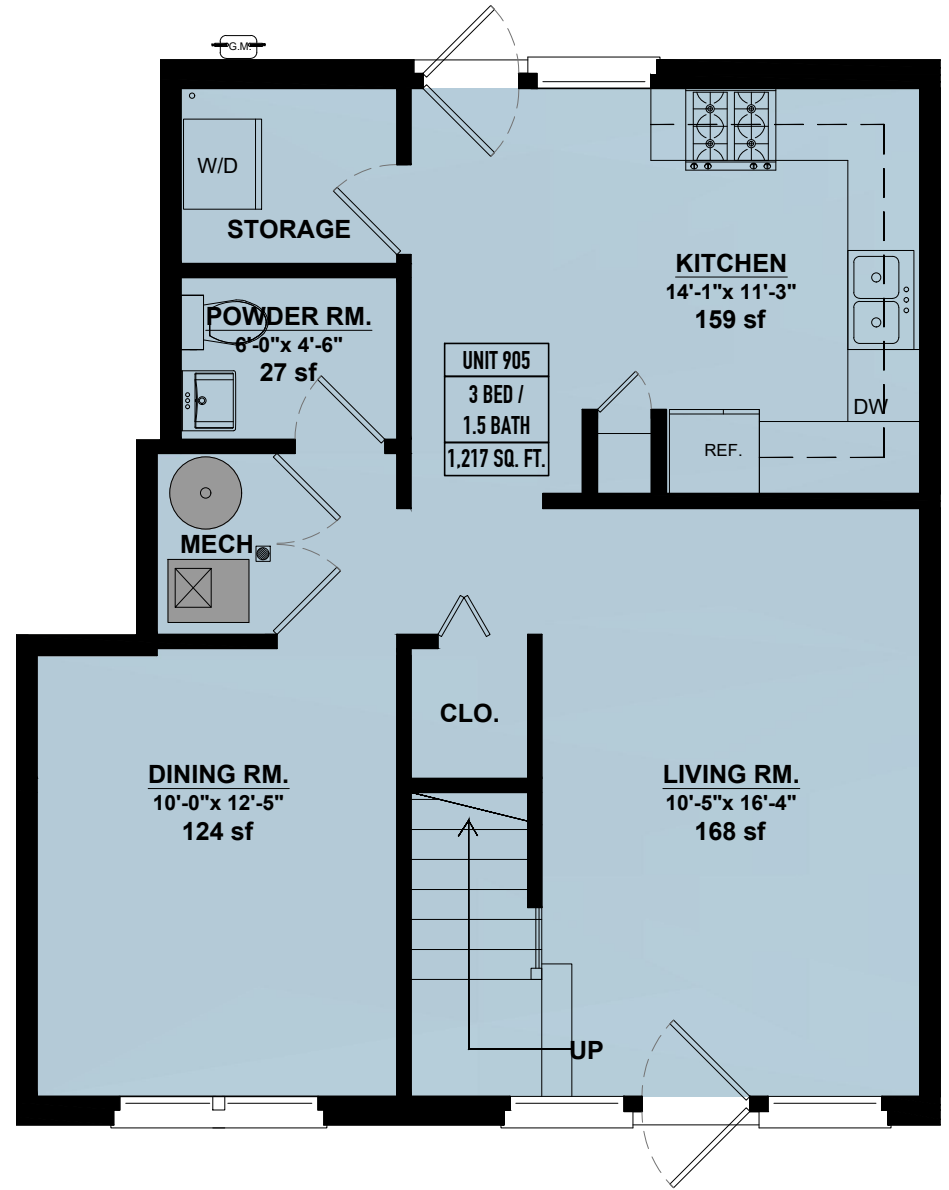
GROUND FLOOR
