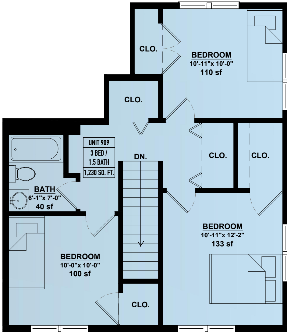
SECOND FLOOR
